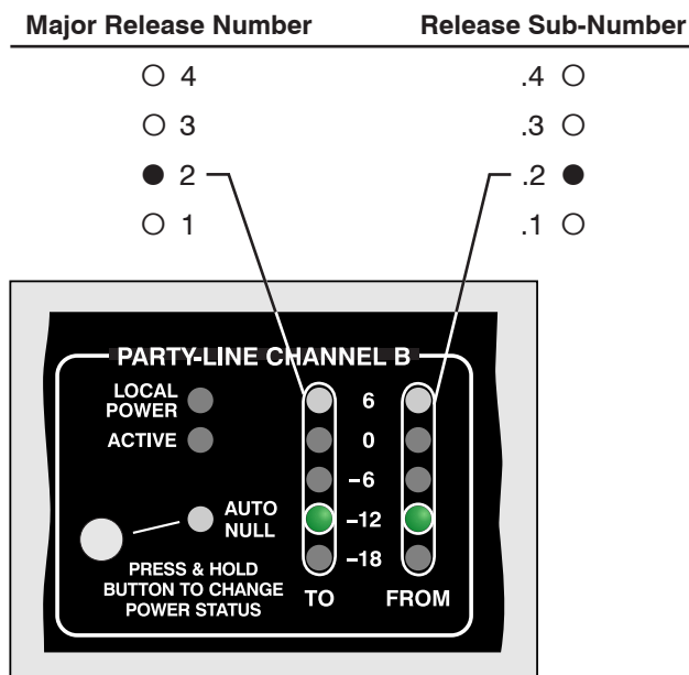
Figure 4. Detail of front panel showing the status LEDs that display the application firmware version. In this example, the application firmware version is 2.2.
