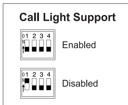
Figure 3. Call light support configuration switch
